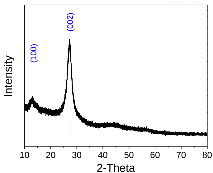
Figure S2. XRD pattern of the g-C 3 N 4 photocatalyst.
