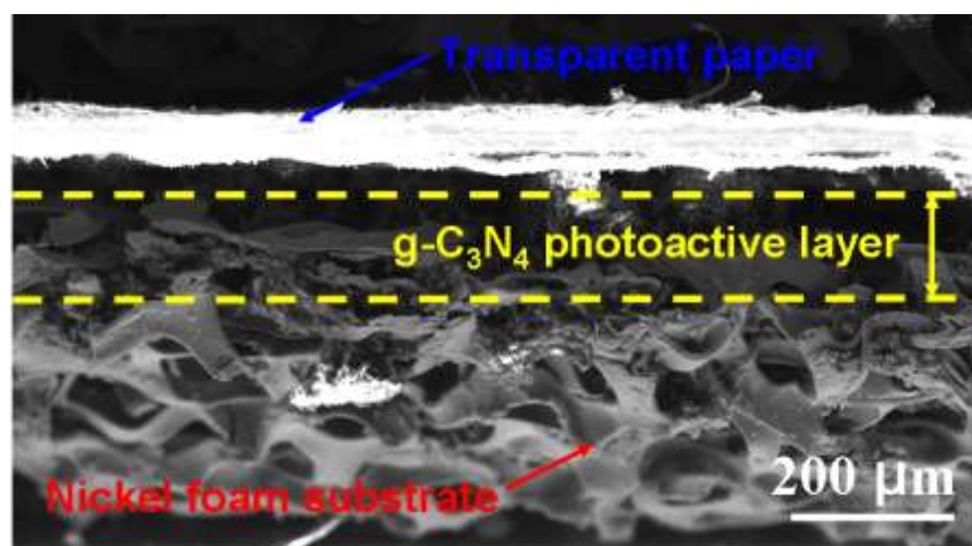
Figure S4. Cross-section SEM image of the sandwich-like photoactive substrate.
