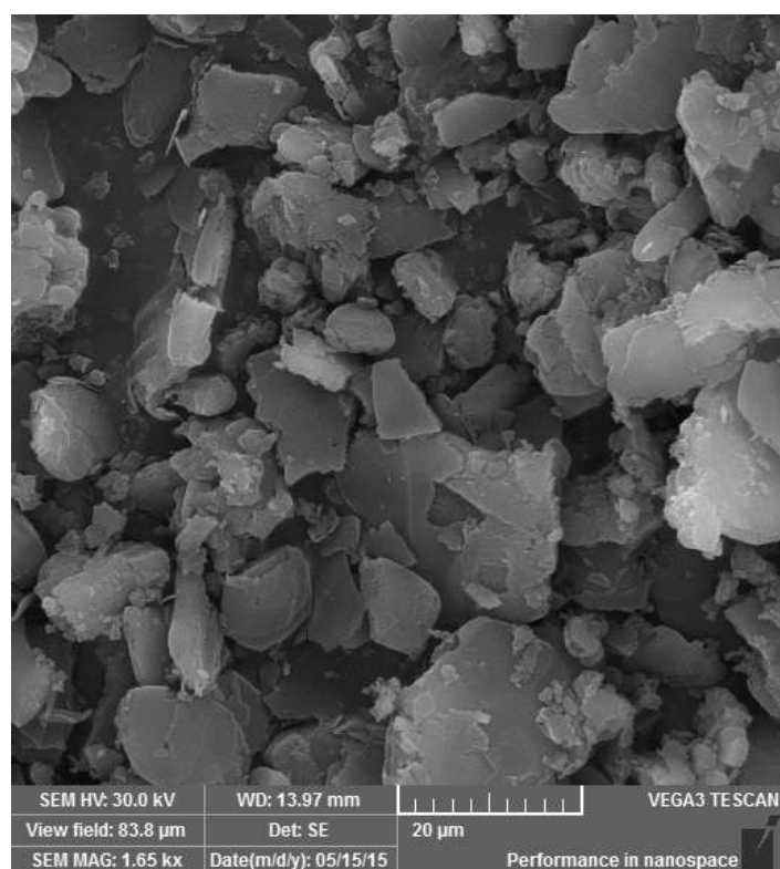
Figure S3. SEM image of the g-C 3 N 4 photocatalyst.
