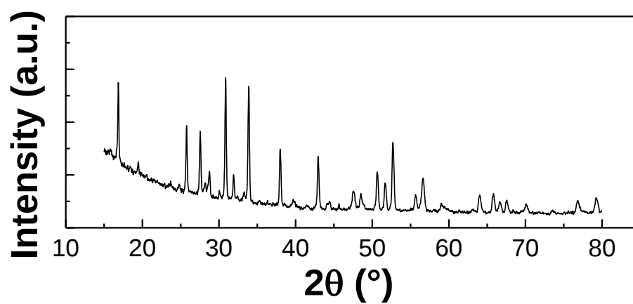
Figure S2. XRD analysis for hybrid electrolyte
