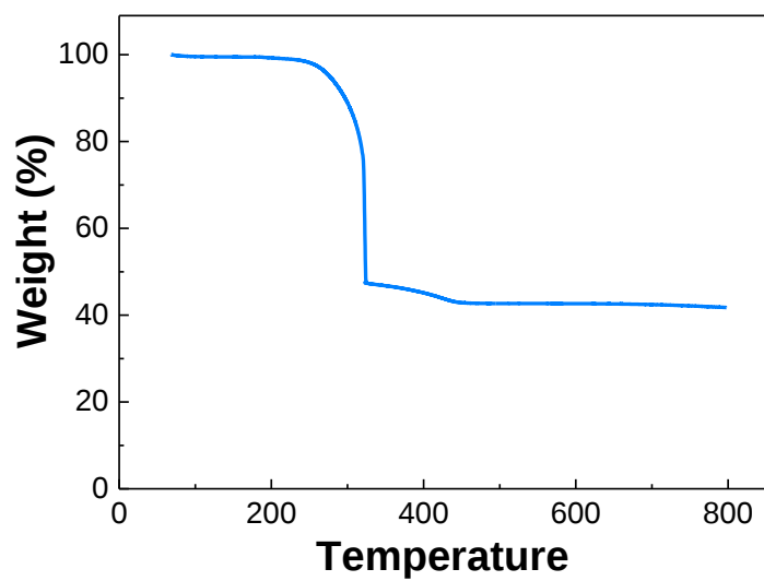
Figure S1. Thermogravimetric analysis (TGA) curve of hybrid electrolyte, which demonstrates good stability below 150 °C
