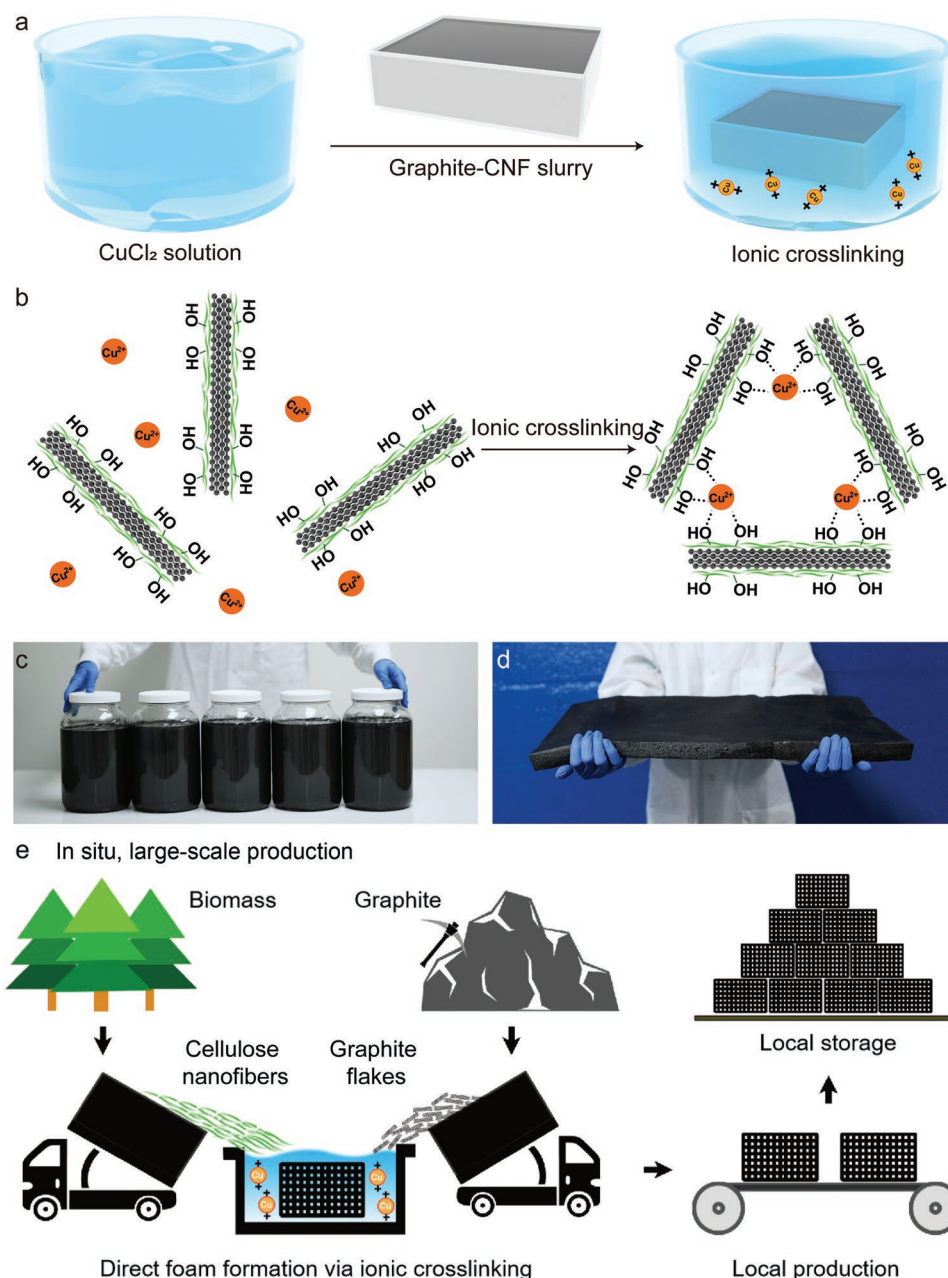
Figure 1. In situ, large-scale production of Cu-G-CNF foams via a freeze-drying-free ionic crosslinking method. a,b) Schematic to show the fabrication process of Cu-G-CNF foam by Cu 2+ ionic crosslinking. c) Large-volume G-CNF slurries produced by sonication, one gallon per bottle. d) A large scale (60 cm × 30 cm × 5 cm) G-CNF foam after air dry. e) The schematic to show the potential application of in situ, large-scale production. The direct foam formation approach via ionic crosslinking treatment holds great promise to produce G-CNF foams on-demand locally (where the foam will be used), avoiding the long-distance transportation of final foam product.
